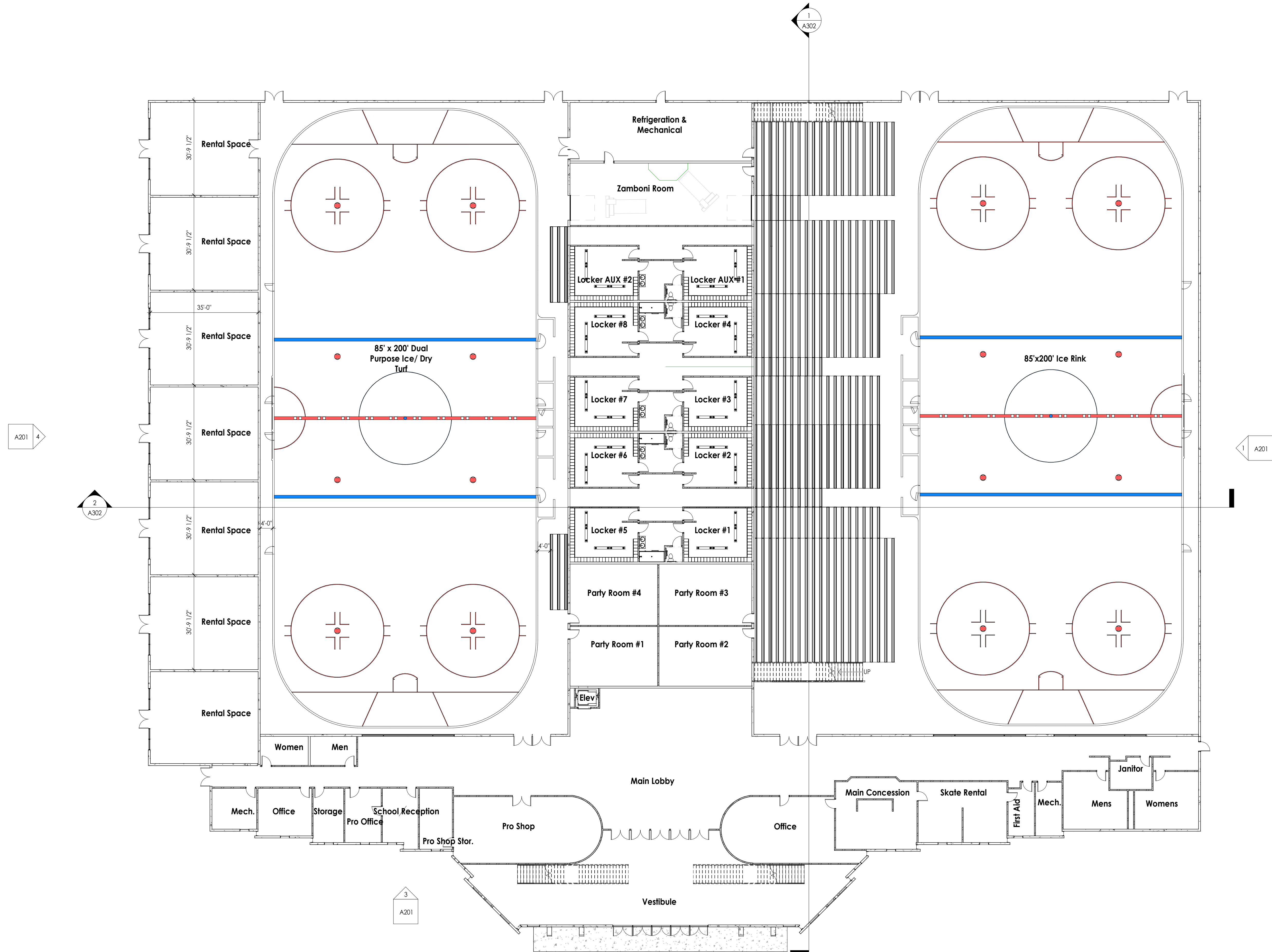
1 MAIN LEVEL FLOOR PLAN SCALE: 1/16" = 1'-0"
